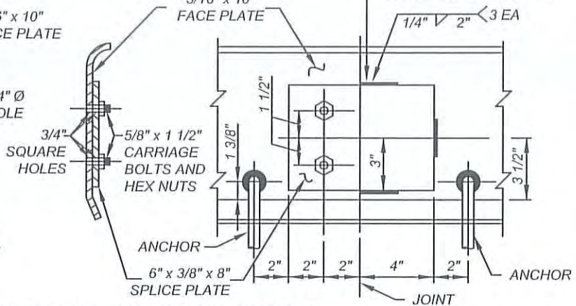
FACE PLATE END AND SPLICE DETAILS
