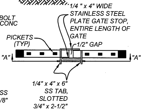
TOP VIEW OF GATE NTS
