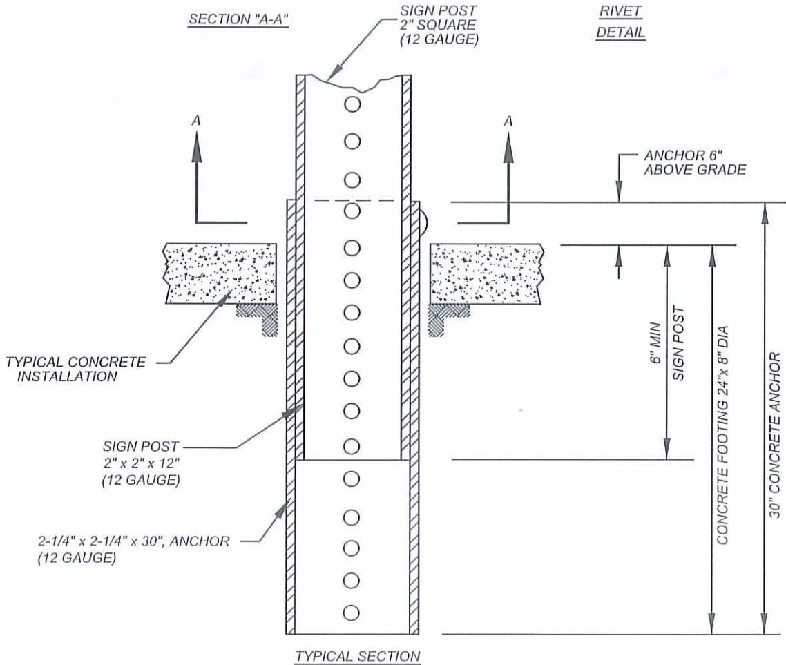
TYPICAL SECTION
